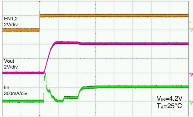
Turn-On in 1x Mode
